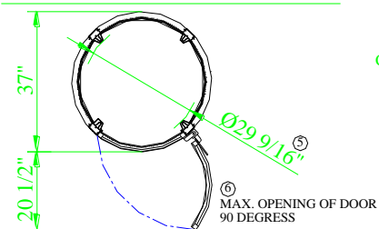
VIEW "A-A"
