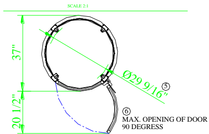
VIEW "A-A"
